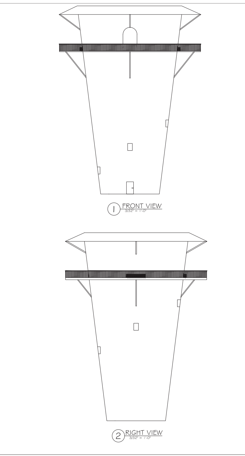
Tower Elevations
