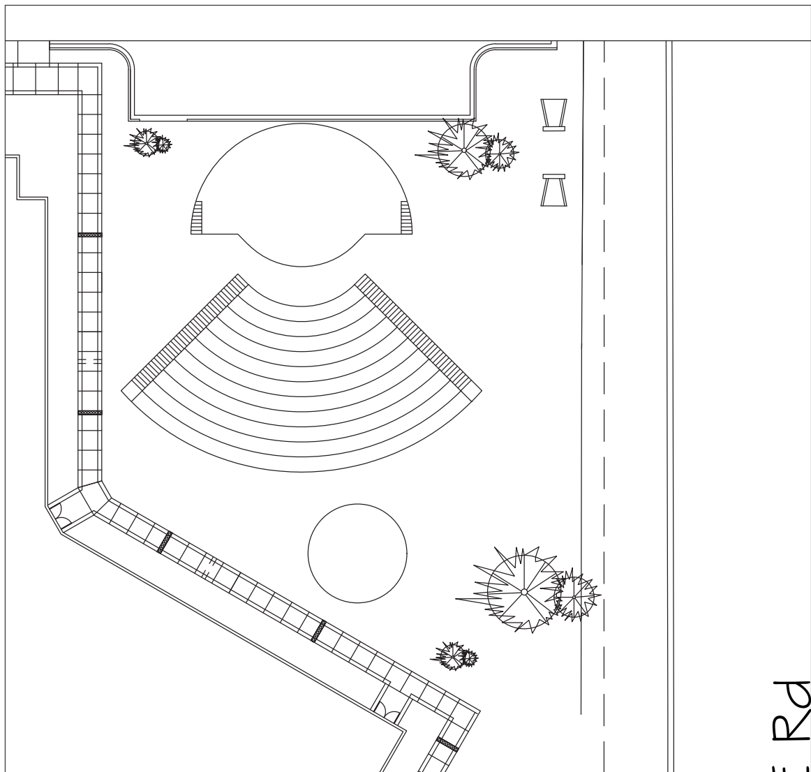
Site Plan
